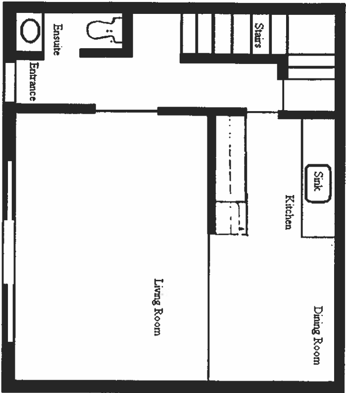
TWO BEDROOM TOWNHOUSE, TYPE C APPROX. 1036 SQ. FT.
